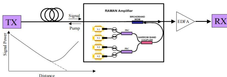
A1600E Raman Amplifier Card (Raman AMP: A1600E-EDFA-R-V-M-T/ A1600E-EDFA-R-V-M-R)
