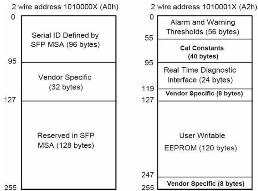
EEPROM Serial ID Memory Contents (A0h)
