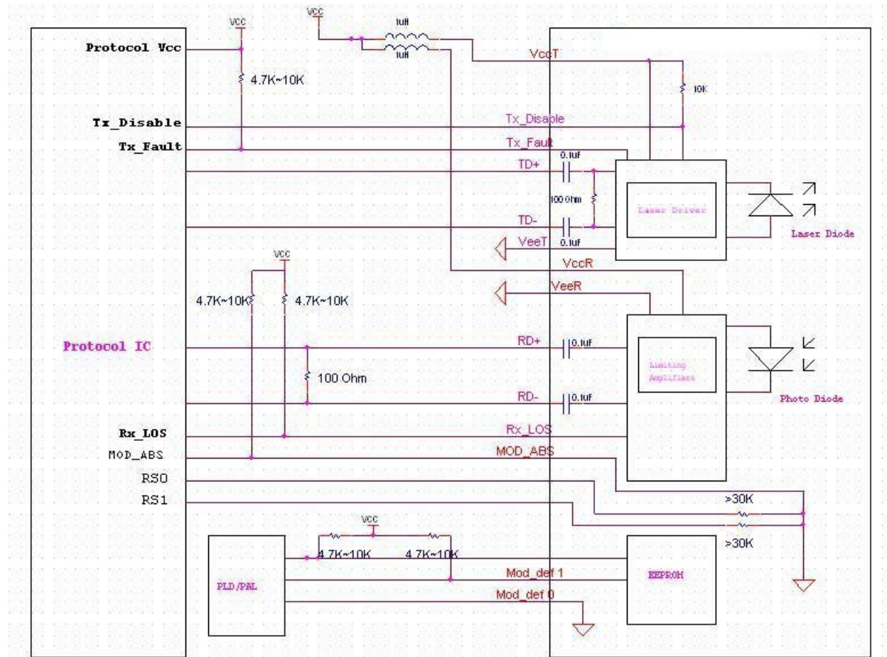
Cable END—SFP+
